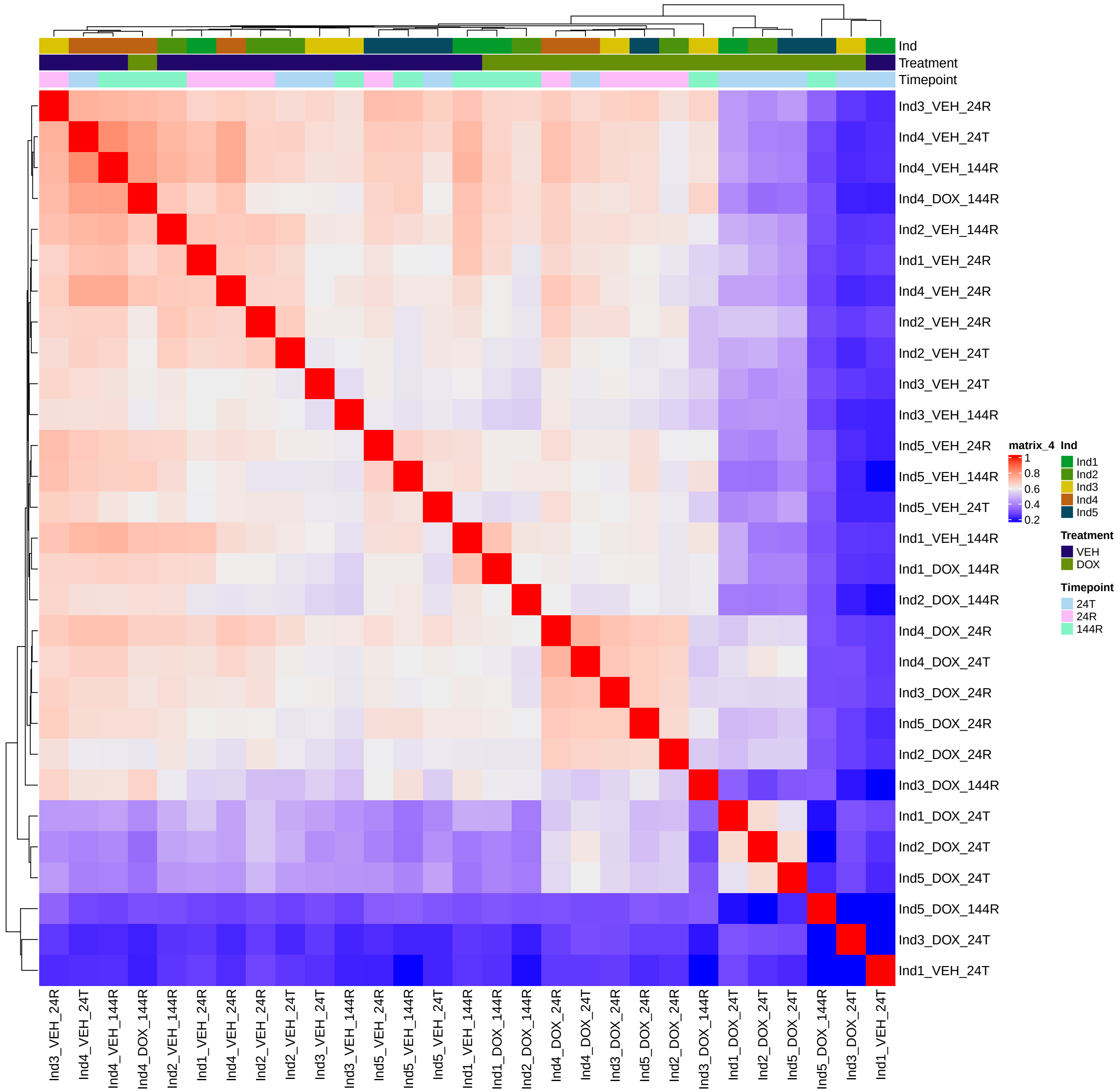
Filtered log2cpm H3K9me3
